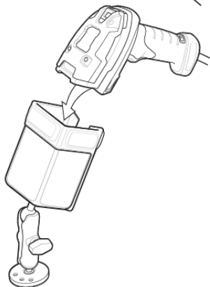
Forklift Holder
